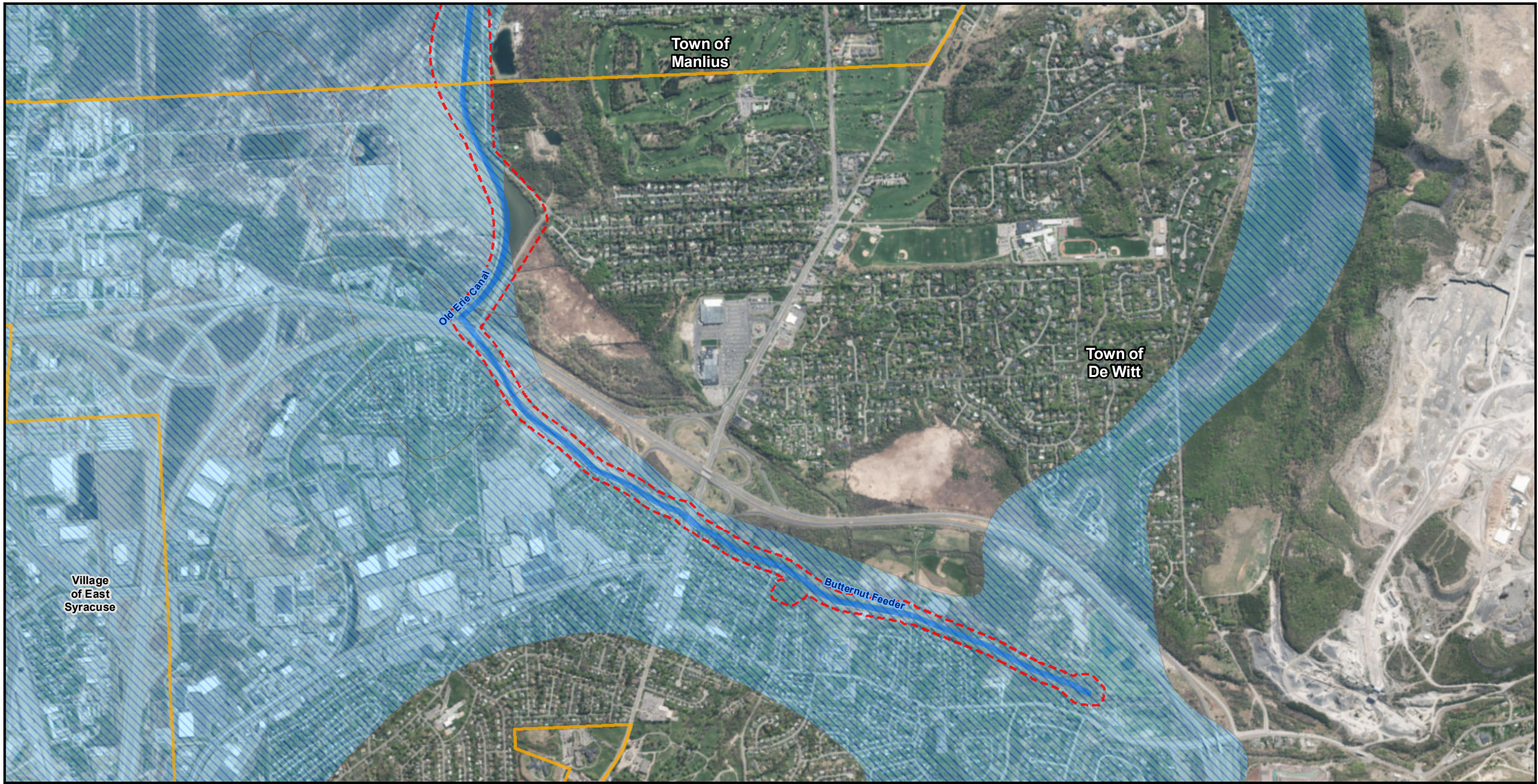
Figure 63F: Aquifers
